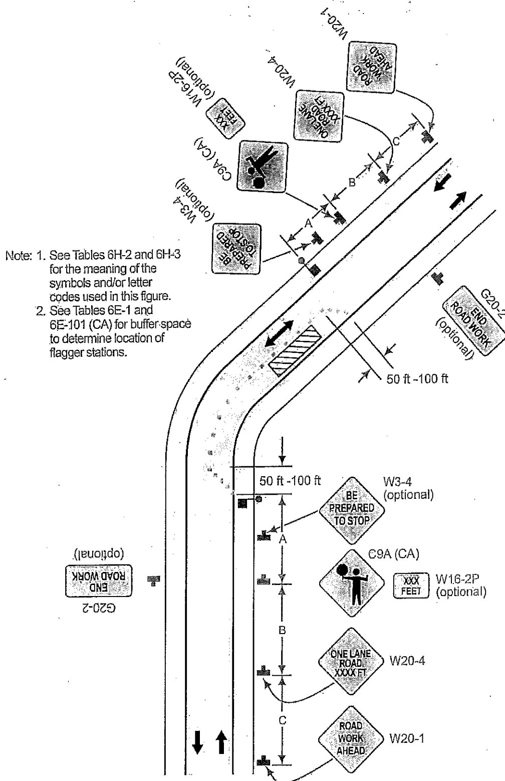
Typical Application 10
